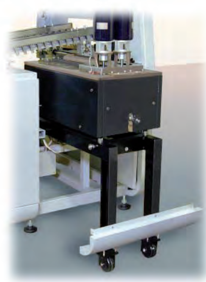
Motorized roll-out pot provides easy access. Pot rolls to front of machine: requires less floor space.
